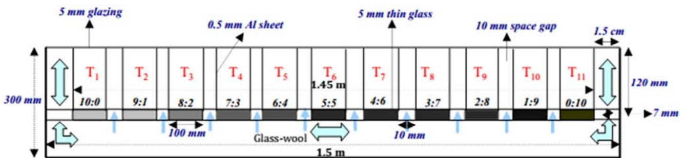
Figure 5. Schematic diagram of experimental set-up of FPSC showing TES mixtures in varying ratio.
